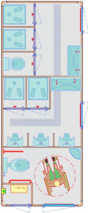
ISO-20Foot-1CC monobloc container equipped with toilets in three areas
