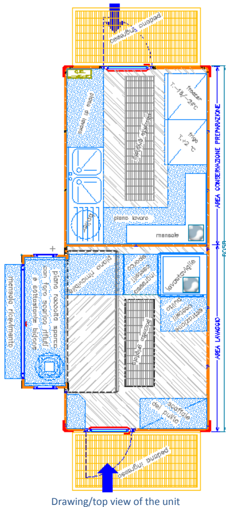
Drawing/top view of the unit
